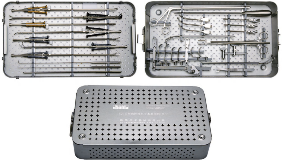
XQ-II型胸腔外科手术器械包(微创瓣膜包) (ZL182) XQ-II type MIS Valve Replacement Instruments Set (ZL182)
